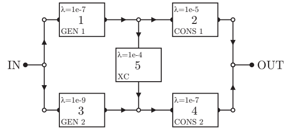
FIGURE 1: Example of an unidirectional bridge structure RBD
