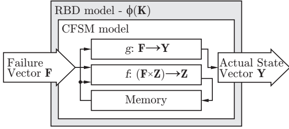
FIGURE 2: CFMS model embedded into RBD model
