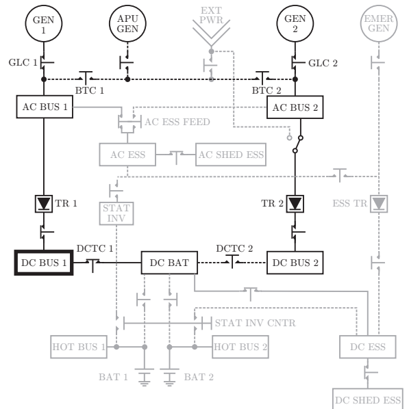
FIGURE 5: ATA 24 system layout of the Airbus A320
