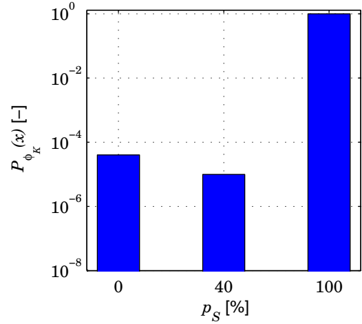
FIGURE 9: PDA based on a first dispatchable system state degradation
