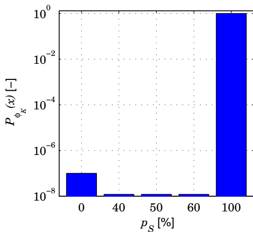
FIGURE 8: PDA based on a nominal system state
