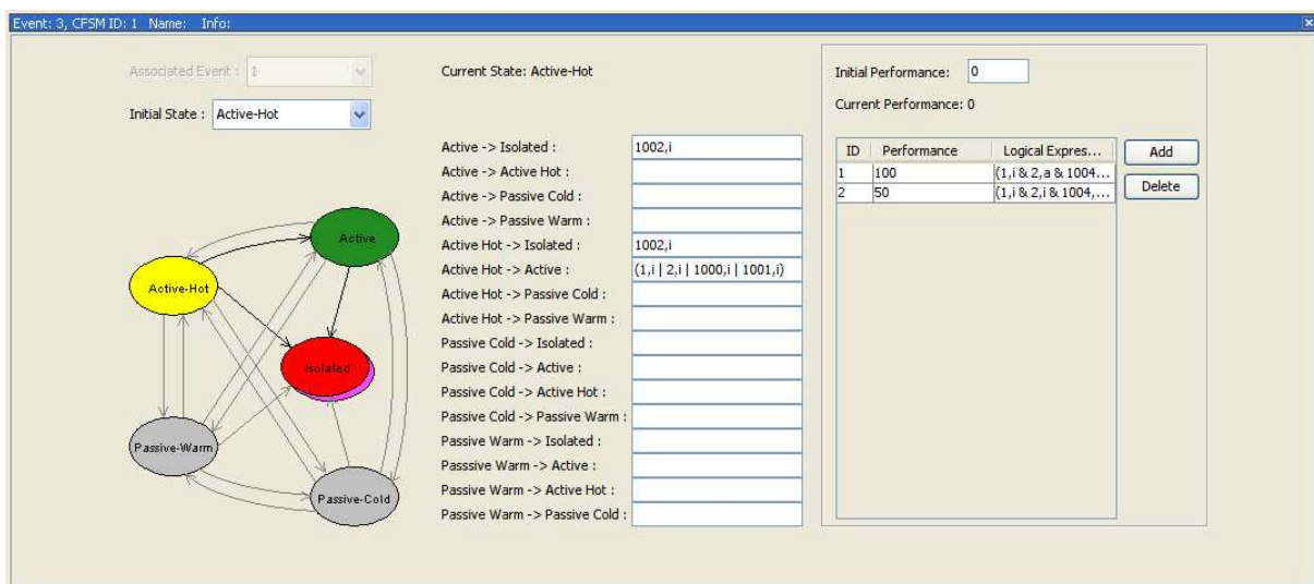
FIGURE 7: Definition of the APU generator CFSM and performance conditions
