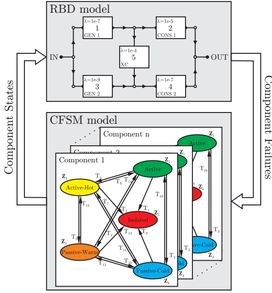
FIGURE 4: Coupling of the RBD and CFMS models
