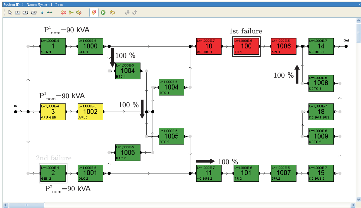
FIGURE 6: RBD for defined TOP EVENT “Power Supply of DC Bus 1”
