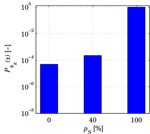
FIGURE 10: PDA based on a second system state degradation
